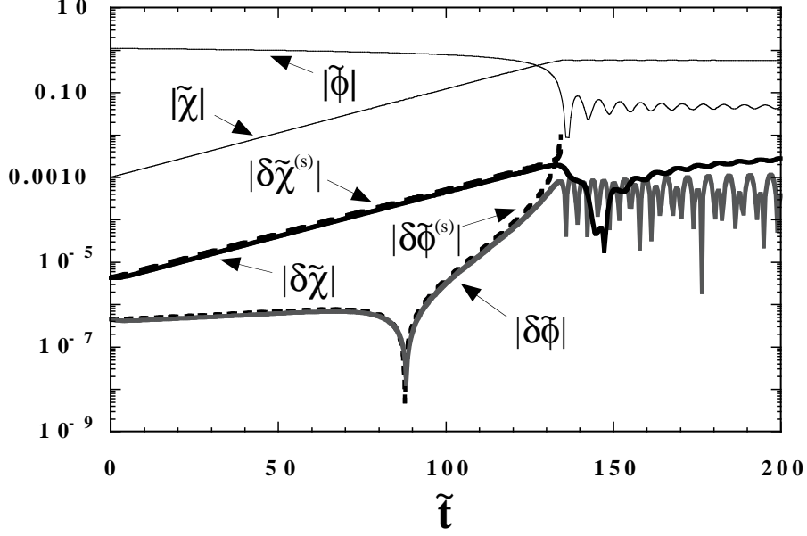
FIG. 4: The evolution of background fields, \tilde{\phi} = \phi/m_{\text{pl}} and \tilde{\chi} = \chi/m_{\text{pl}} , and long-wave field perturbations, \delta\tilde{\phi} \equiv k^{3/2}\delta\phi/m_{\text{pl}} and \delta\tilde{\chi} \equiv k^{3/2}\delta\chi/m_{\text{pl}} as a function of time, \tilde{t} \equiv m_{\text{pl}}t/\sqrt{96\pi q} in the R^2 inflationary scenario with a non-minimally coupled \chi field for \xi = -0.025 . The initial values of scalar fields are chosen as \phi_* = 1.1m_{\text{pl}} and \chi_* = 10^{-3}m_{\text{pl}} . We also plot the slow-roll results, where we denote \delta\tilde{\phi}^{(s)} and \delta\tilde{\chi}^{(s)} in the figure. The evolution of \delta\tilde{\phi}^{(s)} and \delta\tilde{\chi}^{(s)} after inflation is not shown.
